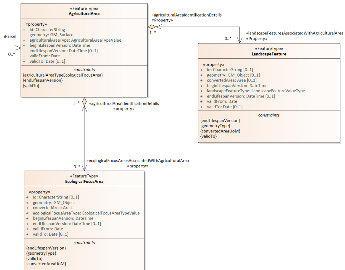
Figure 3. LPIS UML model - AgriculturalArea, LandscapeFeature and EcologicalFocusArea class diagrams and relationships
