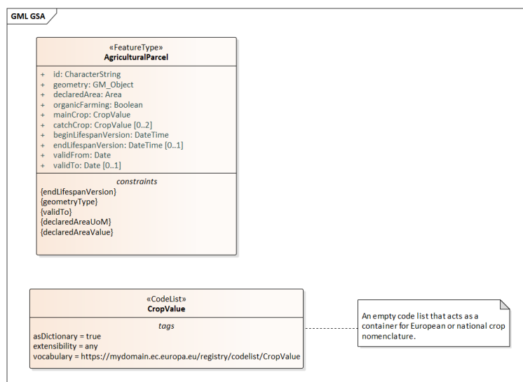
Figure 9. GSA UML model
