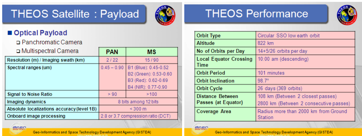
Figure 3 - The THEOS payload and performance
