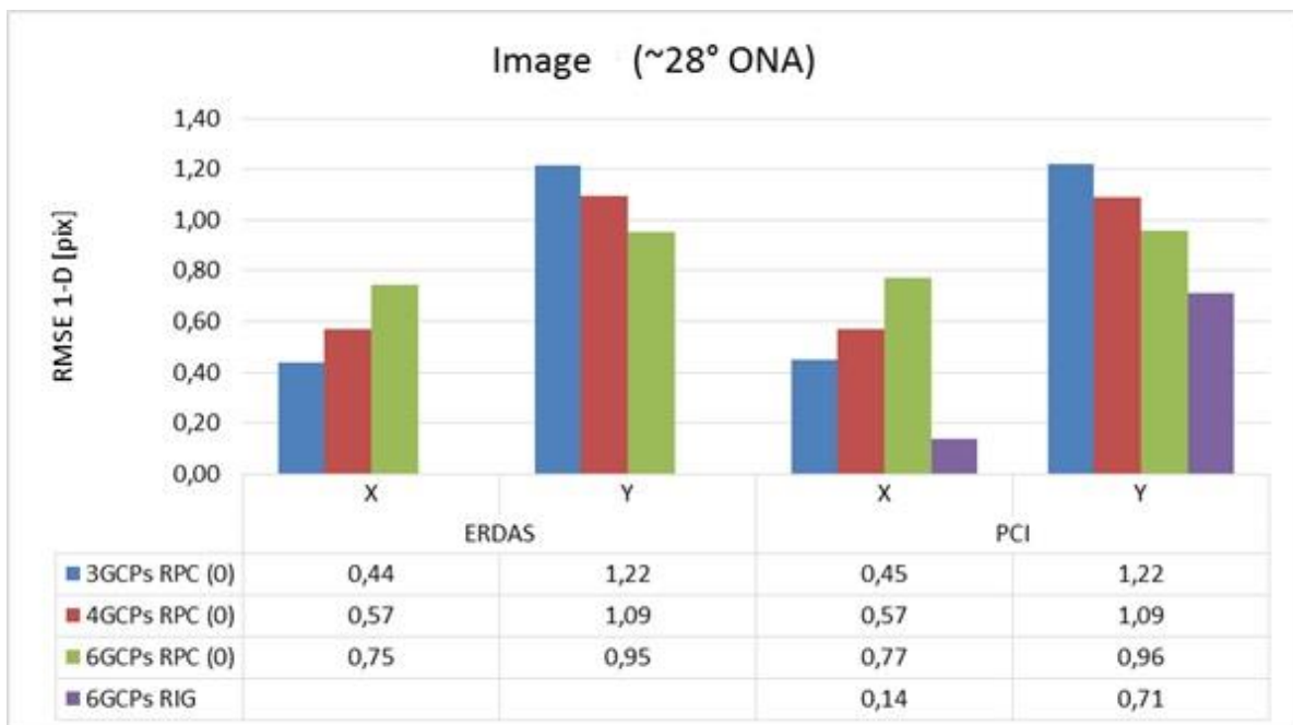
Figure 6 Residuals obtained in phase 1 – image ( \sim 28^\circ ONA)
