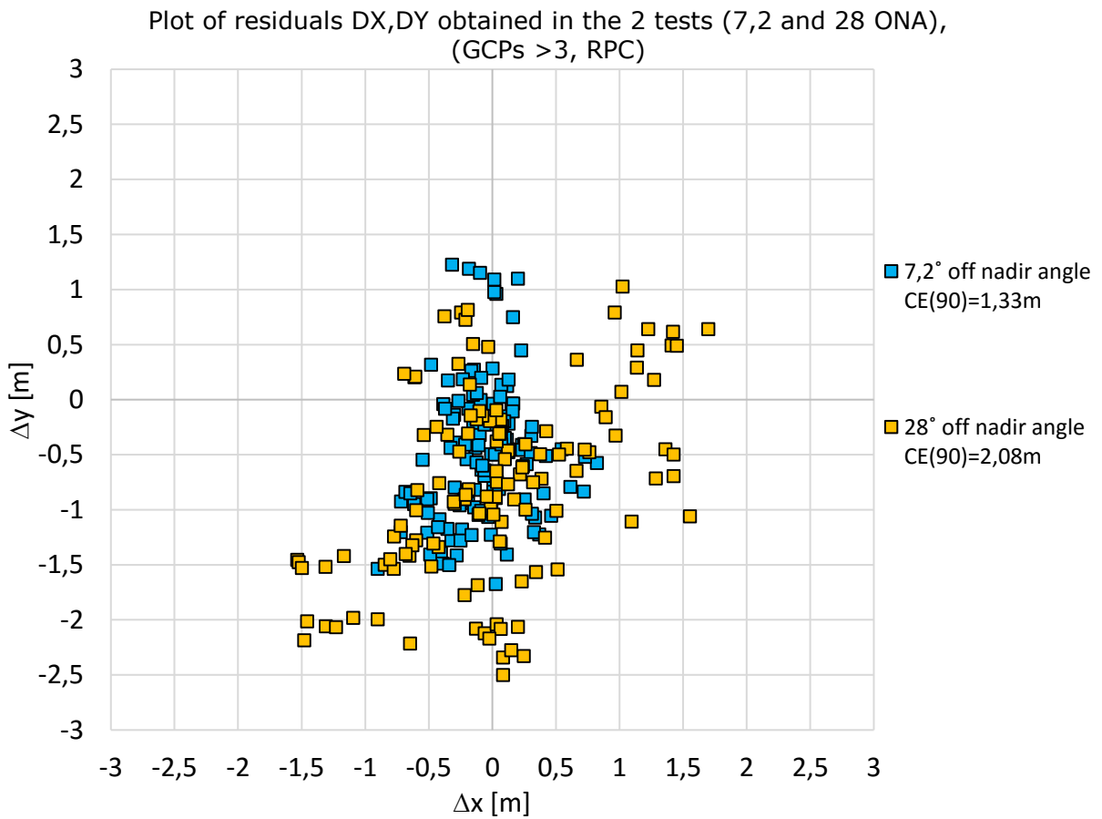
Figure 10 Point representation of planimetric residuals measured on orthoimages based on RPC modelling using JRC ICPS dataset
