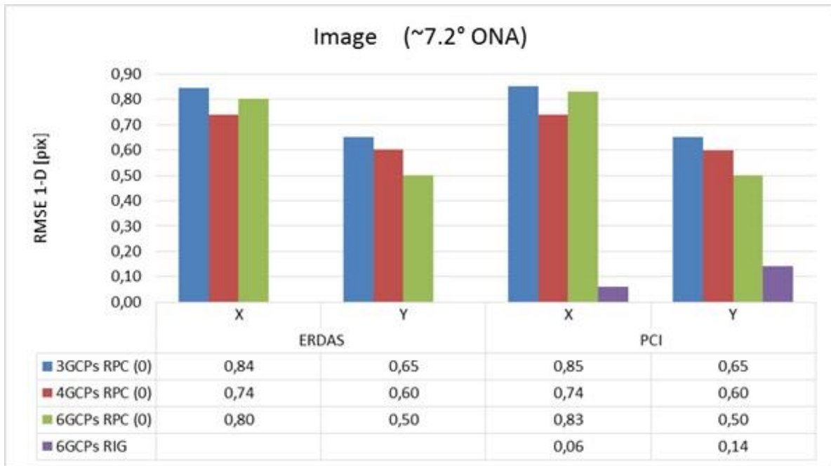
Figure 5 Residuals obtained in phase 1 – image ( \sim 7.2^\circ ONA)
