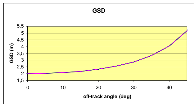
Fig. 3 - GSD at, at Nadir, is 2m PAN, and 8m MSP (off-nadir angles in all JRC studies performed cause cross track GSD(X) resolution to vary between 2.025 - 3.104m
