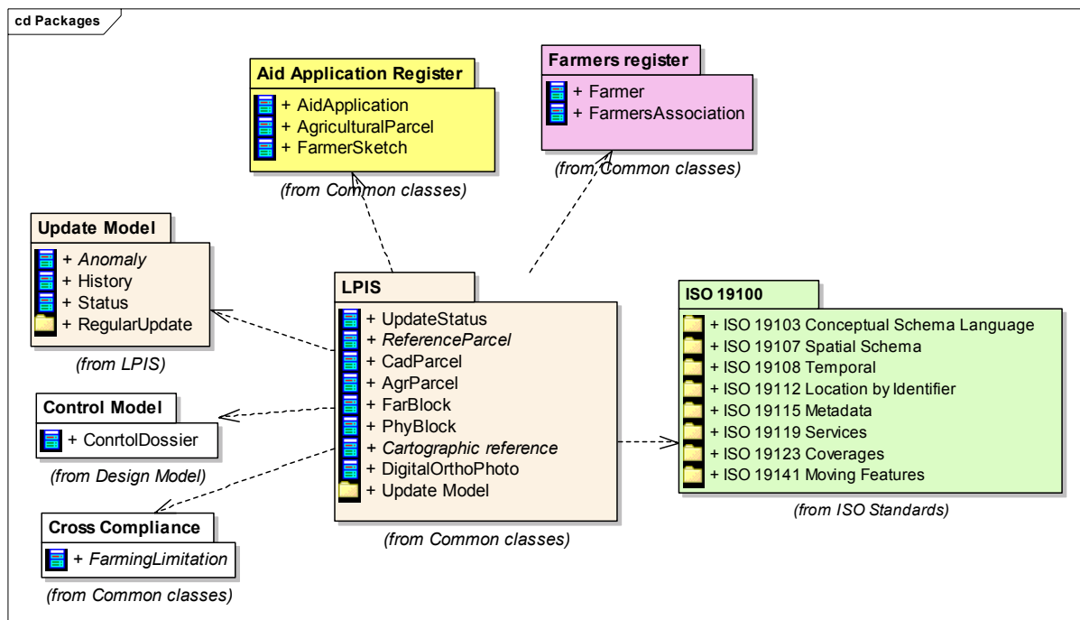
Figure 13. Packages diagram
