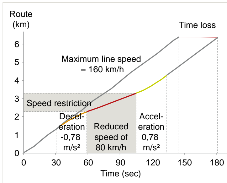
Figure 9: Time loss due to speed restriction
