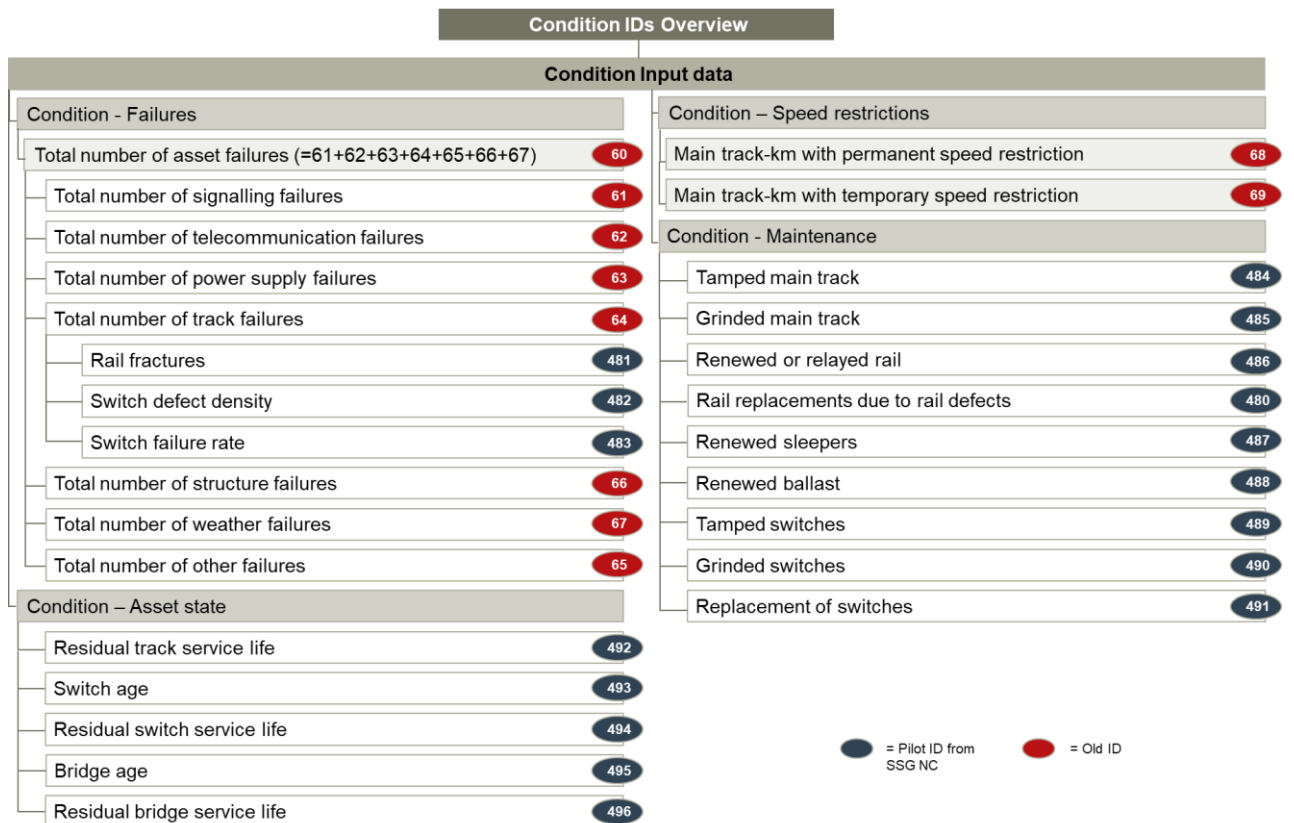
Figure 6 PRIME Input Data Items, basis for condition KPI
